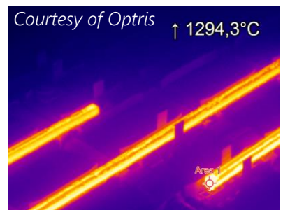
Courtesy of Optris ↑ 1294,3°C Fig1 : Thermographic image of steel slabs captured with P11M
