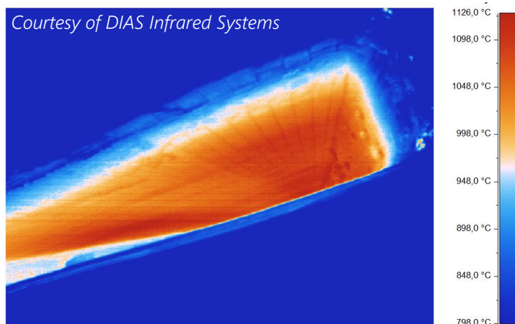
Fig4 : Non-contact temperature measurement in combustion chambers
